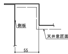
D部詳細 (1:5)
